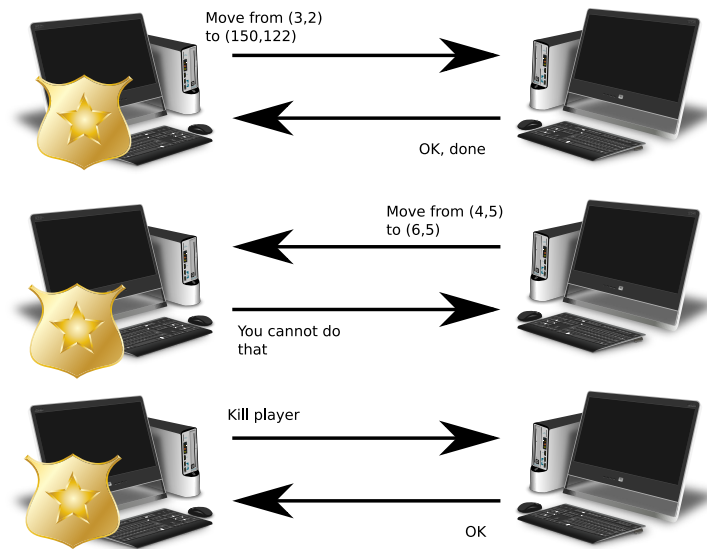
Figure 432: What would happen if one of the Peers had the authoritative game state
